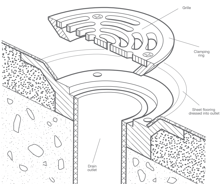
Transition with clamping drain
