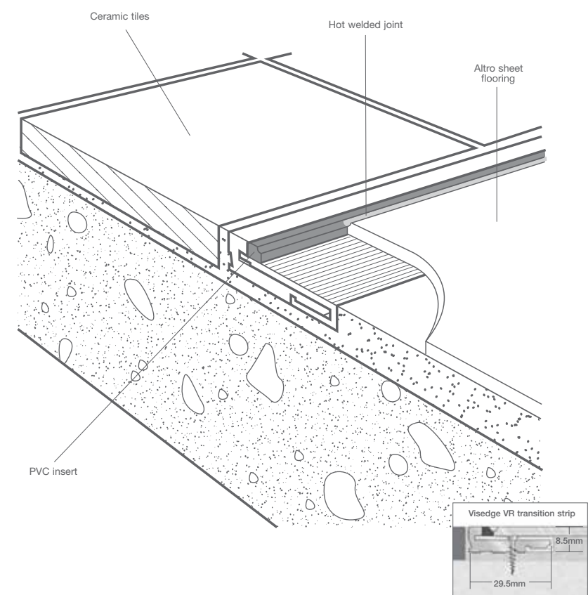
Transition with other floor surfaces
