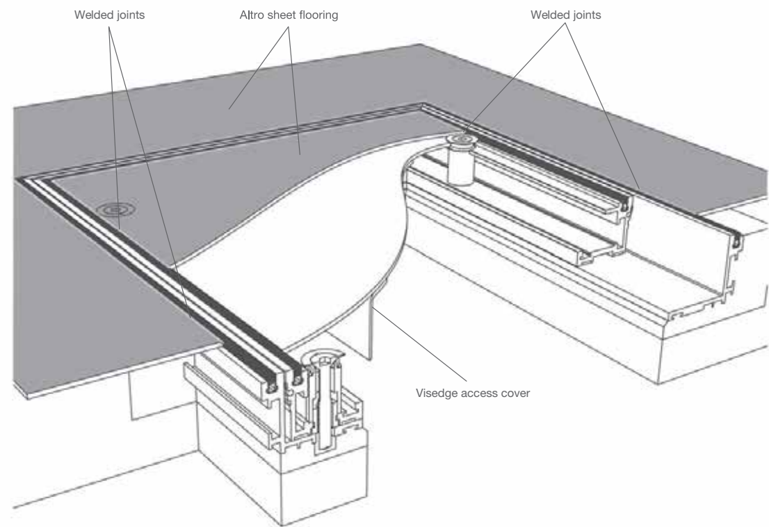
Transition with access covers
