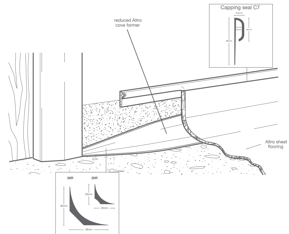
Self-coved to architrave
