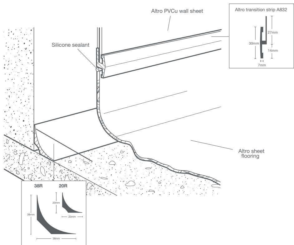
Self-coved to architrave
