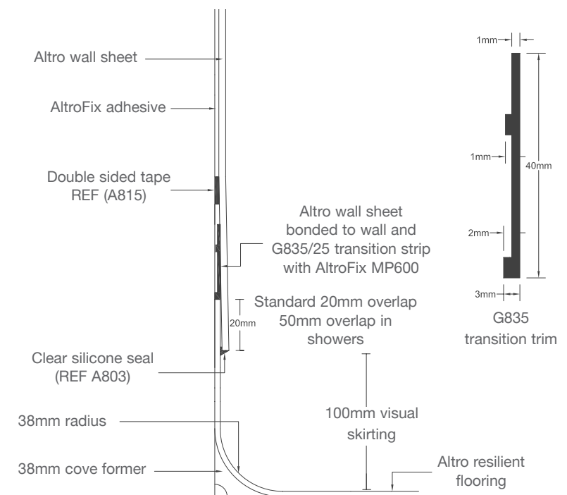
Concealed transition strip
