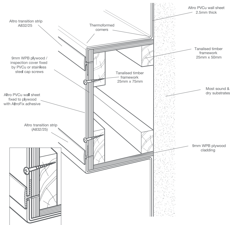
Altro Whiterock hygienic PVCu wall system to Altro flooring for wet environments shower tray detail
